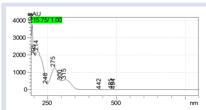
Figure 2: UV-VIS chromatogram of compound-1.
