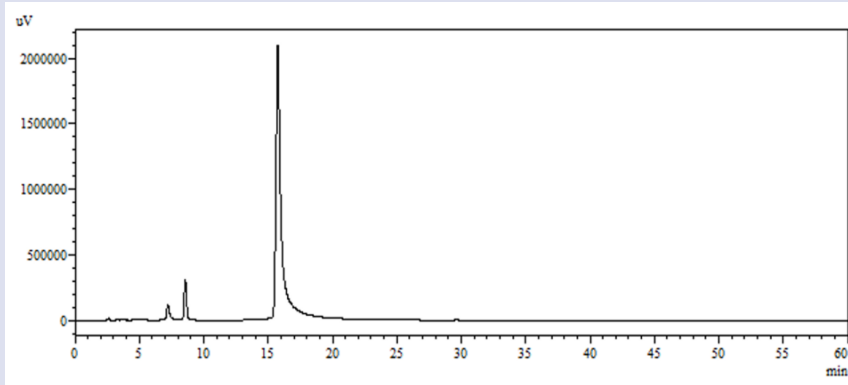
Figure 1: HPLC Chromatogram of compound 1.
