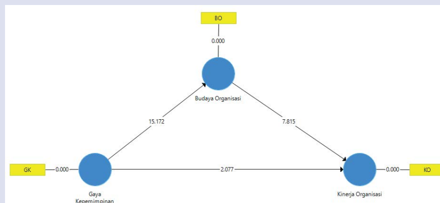
Figure 1. Output Bootstrapping
